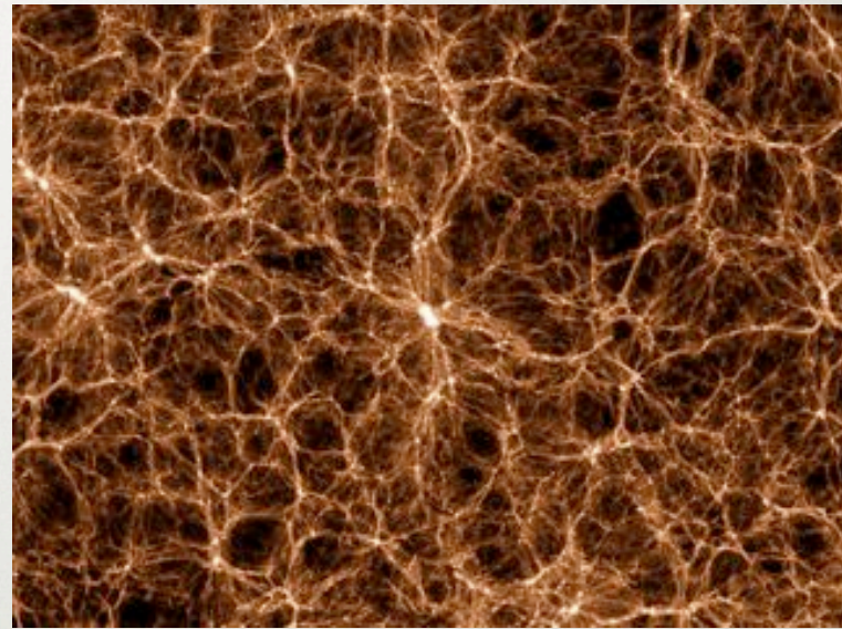
Structure of the Universe: 1 billion light years across
