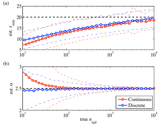
FIG. 6 (color online) Convergence of estimates for (a) x_{\min} and (b) \alpha as a function of the number n_{\text{tail}} of observations in the power-law region, for both continuous and discrete variables. (Standard deviations of the estimates are shown as the dashed lines.) The large deviations for the continuous estimator and small n_{\text{tail}} are due to finite-size sample effects. In general, we find that our parameter estimates appear to be asymptotically consistent, i.e., as n_{\text{tail}} \rightarrow \infty , both \hat{x}_{\min} \rightarrow x_{\min} and \hat{\alpha} \rightarrow \alpha .
