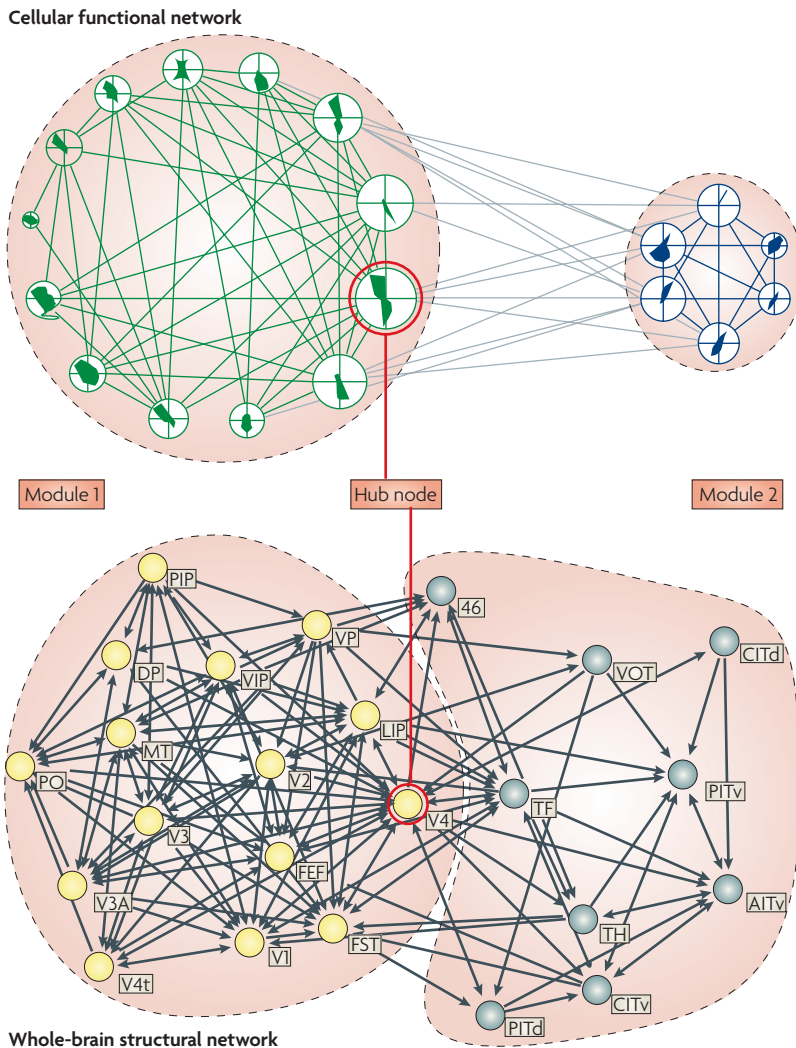
Figure 2 | Cellular and whole-brain networks demonstrate consistent topological features. The top panel shows a cellular functional network constructed from multi-electrode-array recordings made in the anesthetized cat; each node (represented by a circle) corresponds approximately to one neuron and the connections represent high functional connectivity between neurons 86 . The different coloured nodes constitute separate clusters or modules. The plots in each circle illustrate cellular responses to stimuli of different orientations, and the circle size corresponds to the degree (number of functional connections) of each node. The bottom panel shows a whole-brain structural network constructed from histological data on the macaque cortex; each node corresponds to a brain area and the connections represent axonal projections between areas 49 . The network has two main modules, shown here with yellow and grey circles corresponding to mostly dorsal and ventral visual regions, respectively. Both networks exhibit the small-world attributes of high clustering and short path length (see BOX 3); both have an exponentially truncated power law degree distribution (see BOX 2), associated with the existence of high-degree ‘hubs’ (V4 in the anatomical network); and both have a community structure characterized by sparse connectivity between modules (each module is enclosed by stippled lines) and linked by hubs (nodes circled in red). AITv, anterior inferotemporal ventral area; CITd, central inferotemporal dorsal area; CITv, central inferotemporal ventral area; DP, dorsal prelunate area; FEF, frontal eye field; FST, floor of superior temporal area; LIP, lateral intraparietal area; MT, middle temporal area; PIP, posterior intraparietal area; PITd, posterior inferotemporal dorsal area; PITv, posterior inferotemporal ventral area; PO, parieto-occipital area; TF, area TF; TH, area TH; V1–4, visual cortical areas 1–4; VIP, ventral intraparietal area; VOT, ventral occipitotemporal area; VP, ventral posterior area. The top panel is reproduced, with permission, from REF. 86 © (2008) Oxford University Press. The bottom panel is reproduced from REF. 49.
