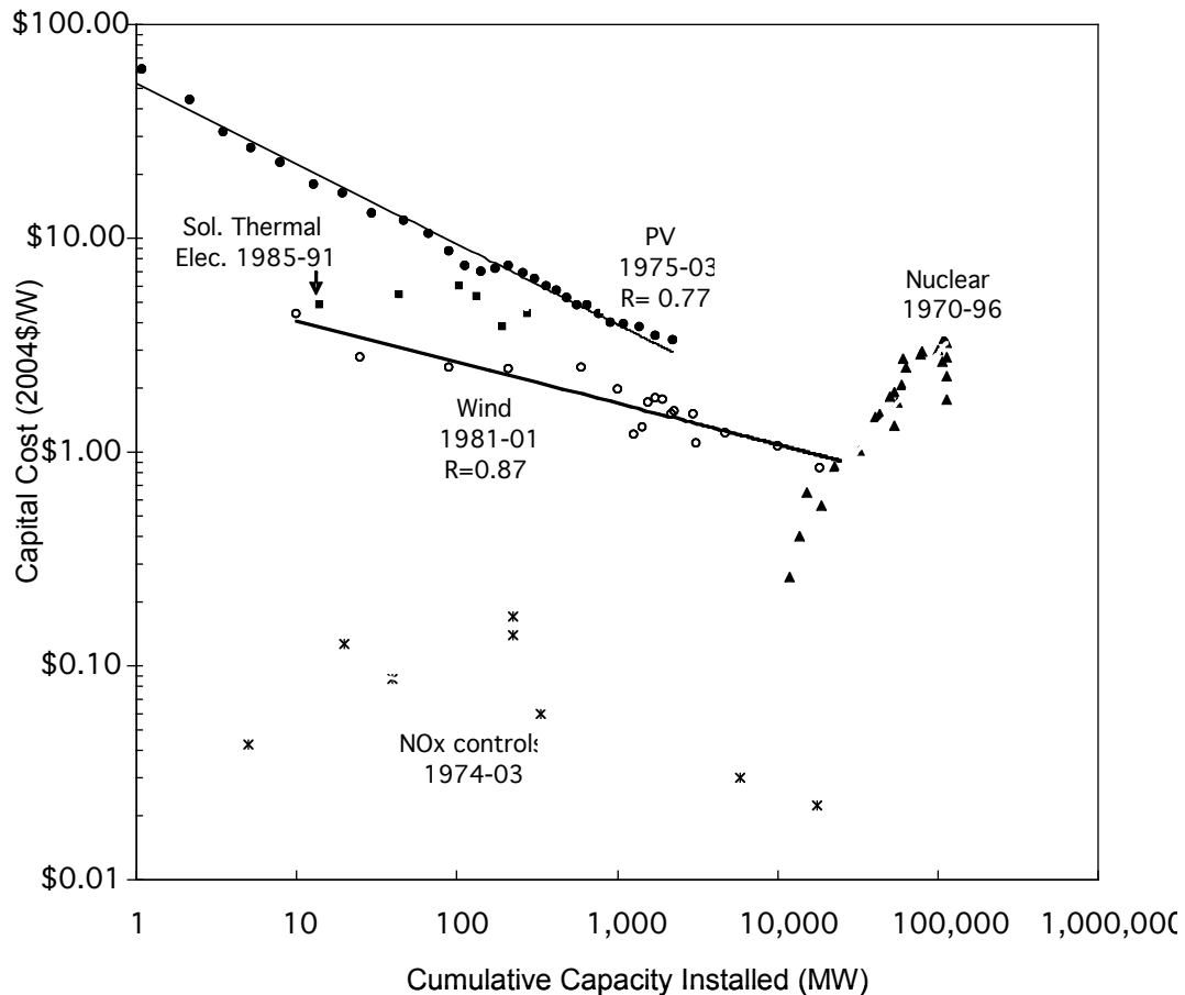
Figure 4. Cost vs. cumulative capacity for electricity generation technologies. Cost is measured in terms of price per watt of peak generating capacity, and cumulative capacity is measured in terms of megawatts of installed capacity. Data is given for wind, PV = photovoltaic, solar thermal, and nuclear power. NOx refers to the additional cost of installing pollution controls that reduce nitrogen oxide to a targeted regulatory level. This data is from selective catalytic reduction (SCR) units installed on natural gas-fired power plants. See [17]. The NOx and nuclear power data are from the US, and the other data sets are global. Several of the data sets are fairly well described by a power law, and the progress ratio (R) is shown for these.
